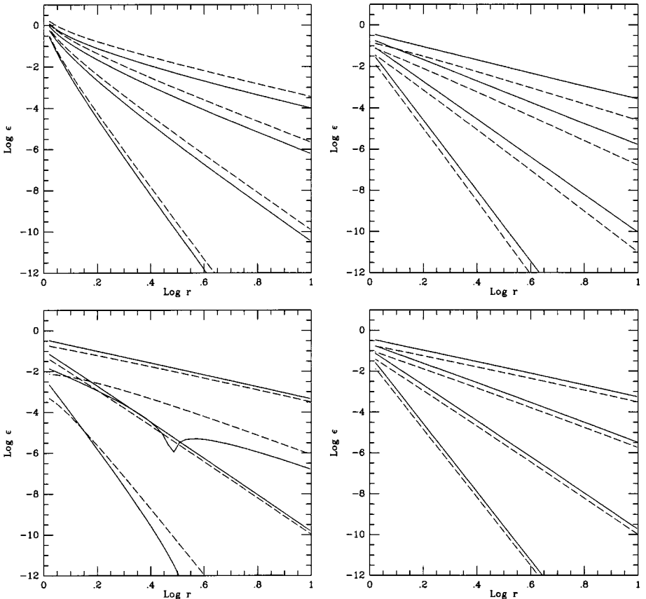
FIG. 2. The absolute error of potential calculated using classical FMM and the pseudoparticle method. The error of the potential by one particle at position (1, 0) is plotted as the function of the distance of r . Solid and dashed curves denote the pseudoparticle method and classical FMM, respectively. In each panel, four curves give the results for p = 2, 4, 8 , and 16 (top to bottom). Four panels are result for the direction angle 0 (top left), 2\pi/3 (top right), \pi/2 (bottom left), \pi (bottom right), respectively.
