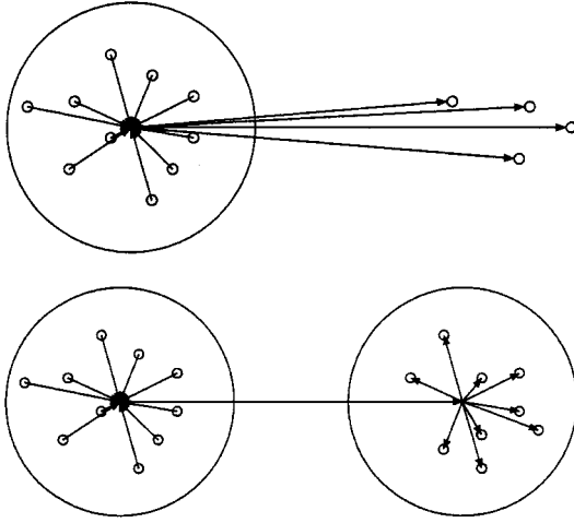
FIG. 1. Approximations in tree (top) and FMM (bottom).
